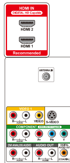
Rear Panel
